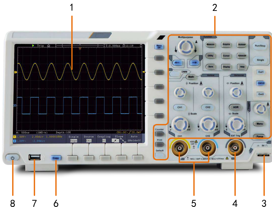
Figure 3-1 Front panel
